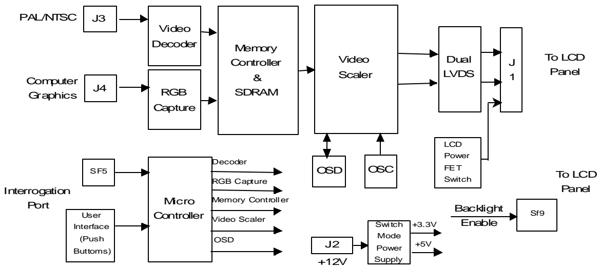
Figure 1-1. VAMP-XGA3 Block Diagram
