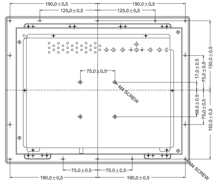
CUT OUT DIMENSION(360x280mm)
