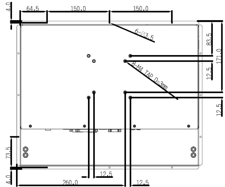
BACK VIEW
