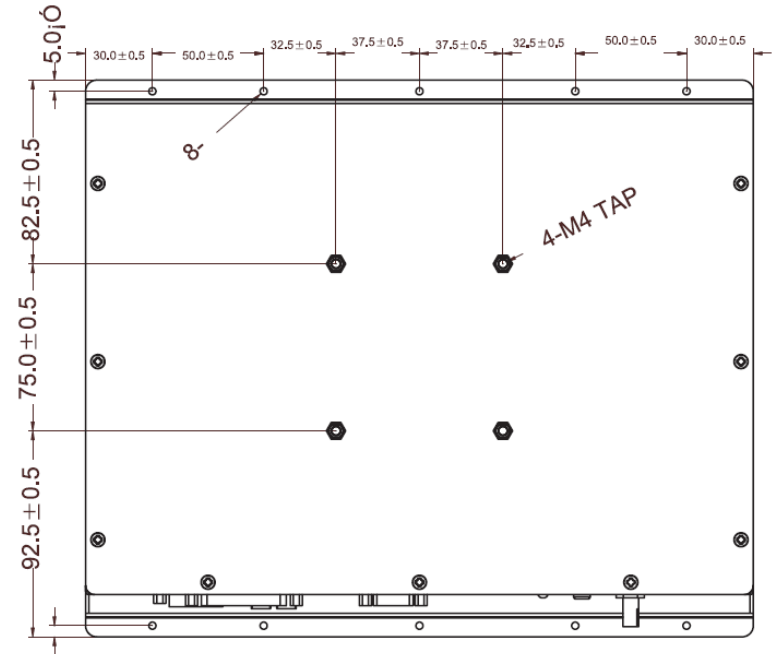
BACK VIEW
